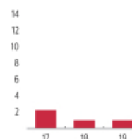
C18 Trading day losses
